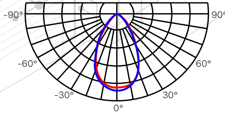
60° Beam Angle
