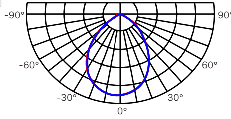
90° Beam Angle
