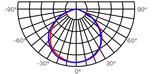
120° Beam Angle
